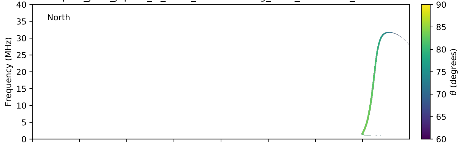
expres_juno_jupiter_io_isaac_lossc-wid1deg_3kev_20161125_v01.cdf
