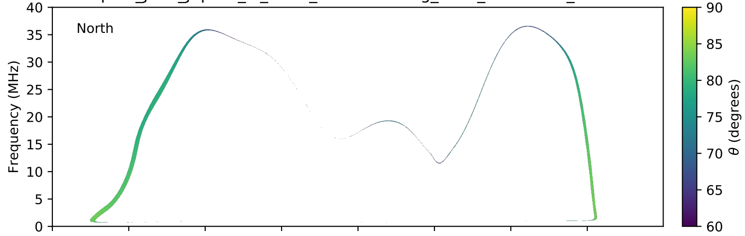
expres_juno_jupiter_io_isaac_lossc-wid1deg_3kev_20161124_v01.cdf
