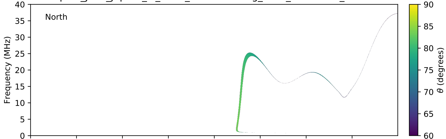
expres_juno_jupiter_io_isaac_lossc-wid1deg_3kev_20161120_v01.cdf
