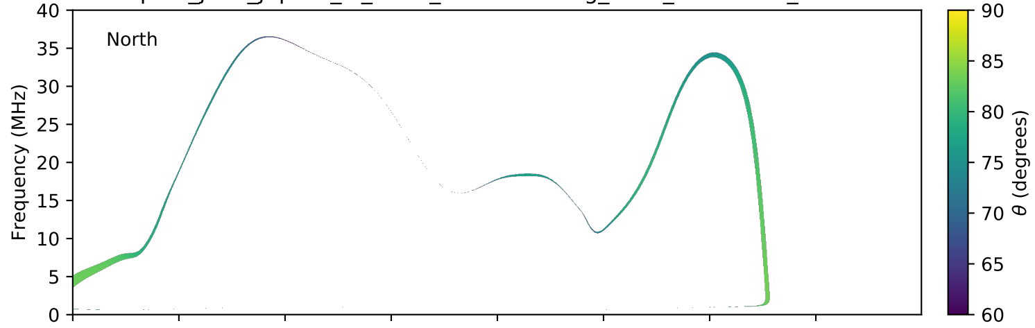
expres_juno_jupiter_io_isaac_lossc-wid1deg_3kev_20161117_v01.cdf
