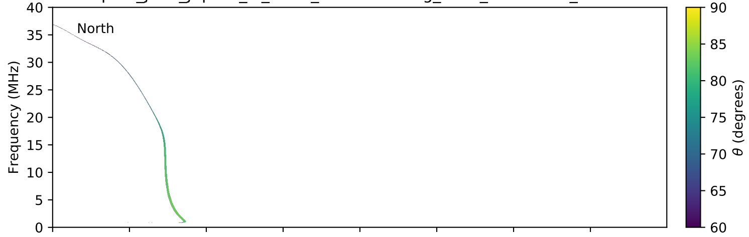
expres_juno_jupiter_io_isaac_lossc-wid1deg_3kev_20161114_v01.cdf
