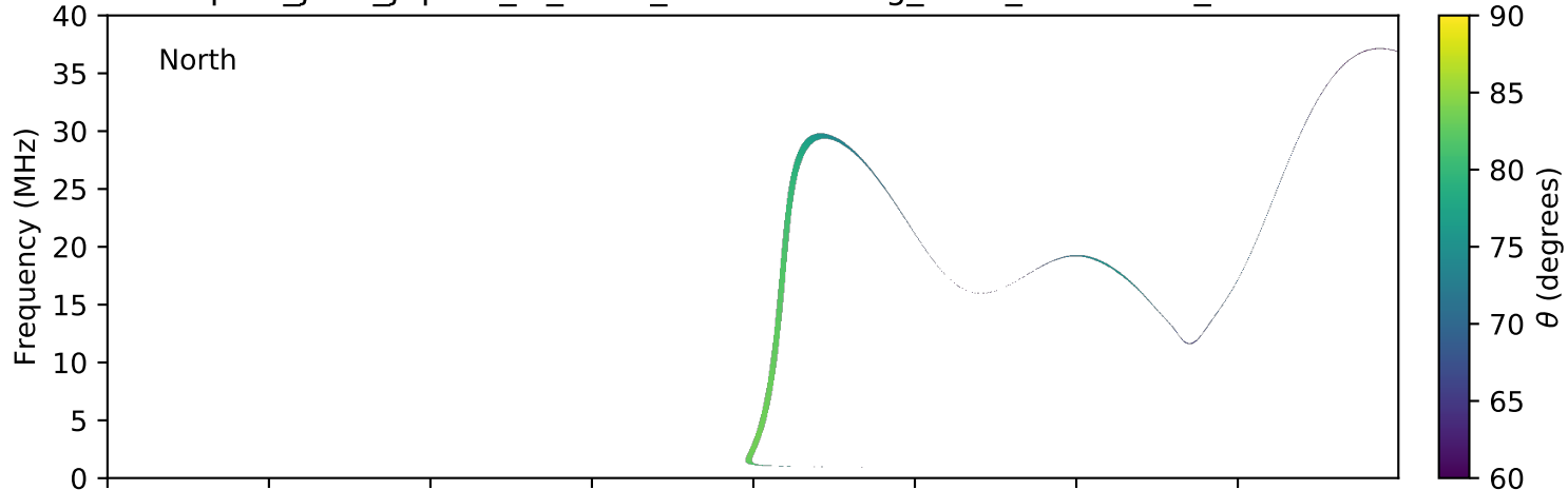
expres_juno_jupiter_io_isaac_lossc-wid1deg_3kev_20161113_v01.cdf
