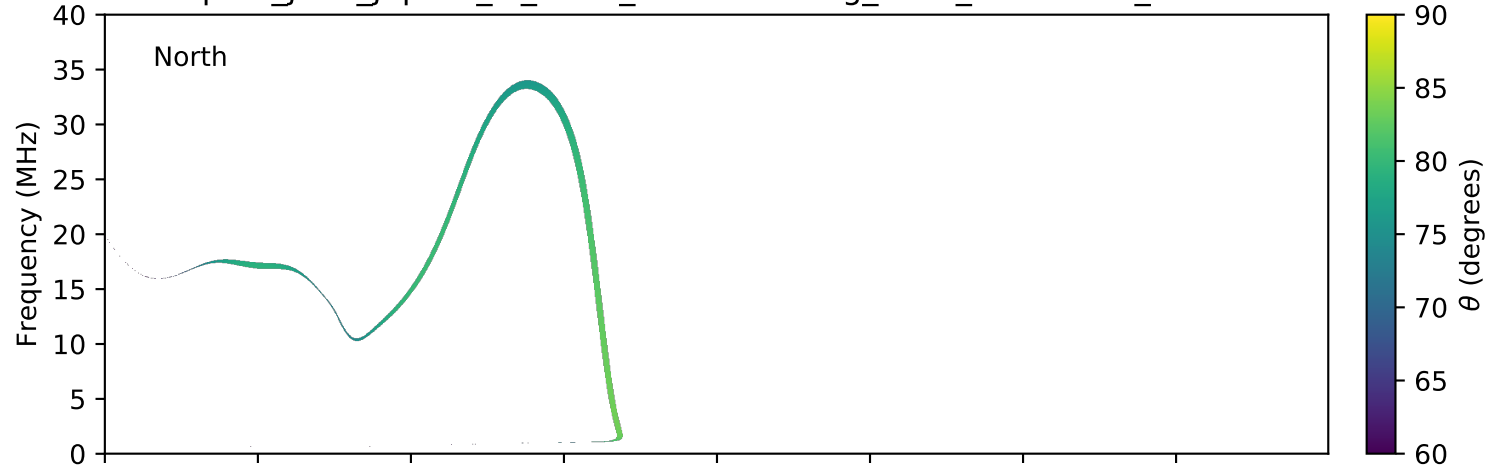
expres_juno_jupiter_io_isaac_lossc-wid1deg_3kev_20161105_v01.cdf
