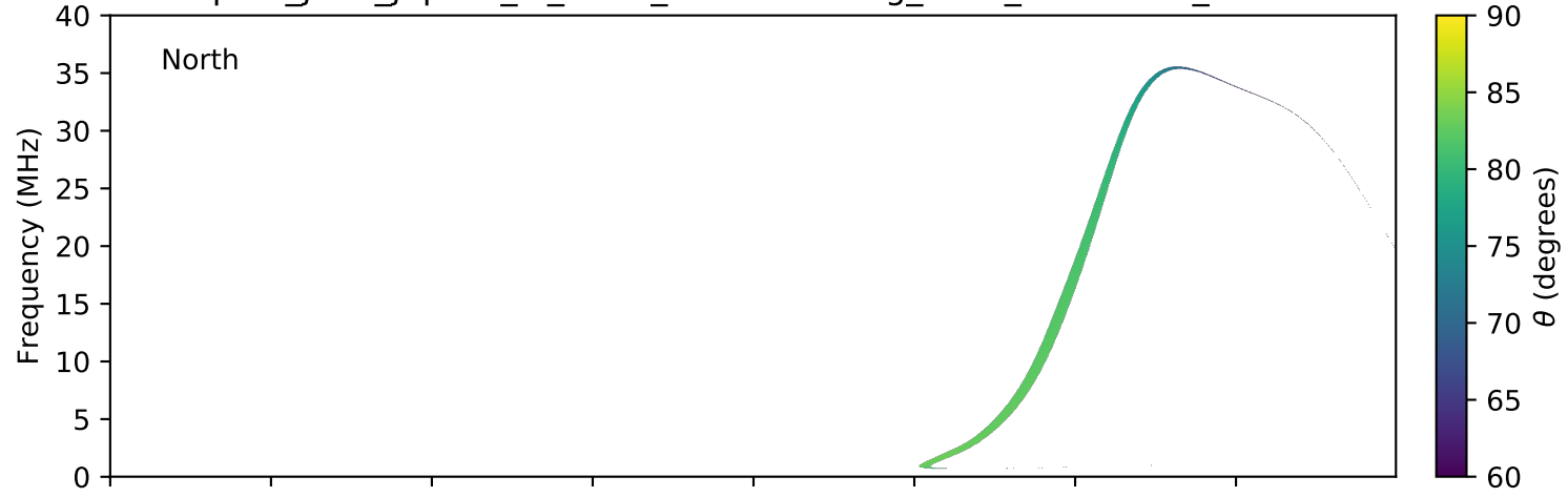
expres_juno_jupiter_io_isaac_lossc-wid1deg_3kev_20161104_v01.cdf
