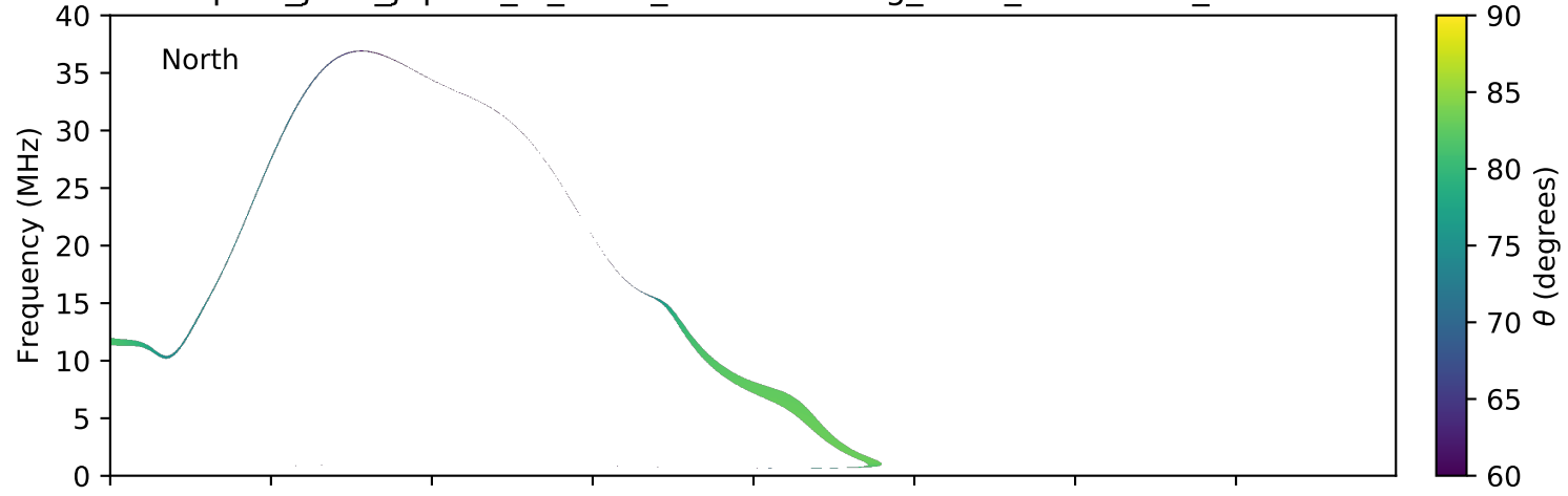
expres_juno_jupiter_io_isaac_lossc-wid1deg_3kev_20161103_v01.cdf
