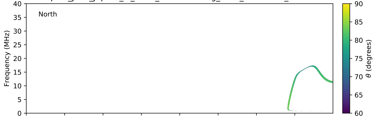
expres_juno_jupiter_io_isaac_lossc-wid1deg_3kev_20161102_v01.cdf
