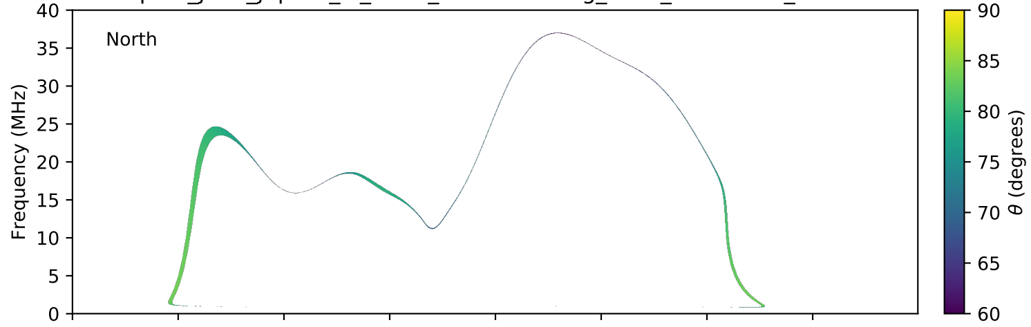
expres_juno_jupiter_io_isaac_lossc-wid1deg_3kev_20161101_v01.cdf
