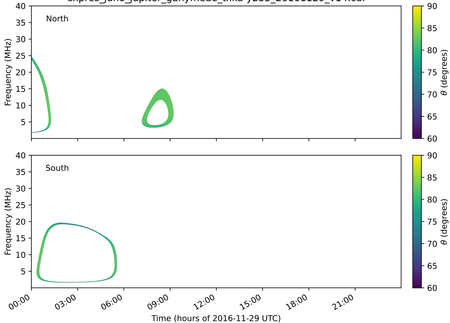
expres_juno_jupiter_ganymede_txka-y235_20161129_v14.cdf
