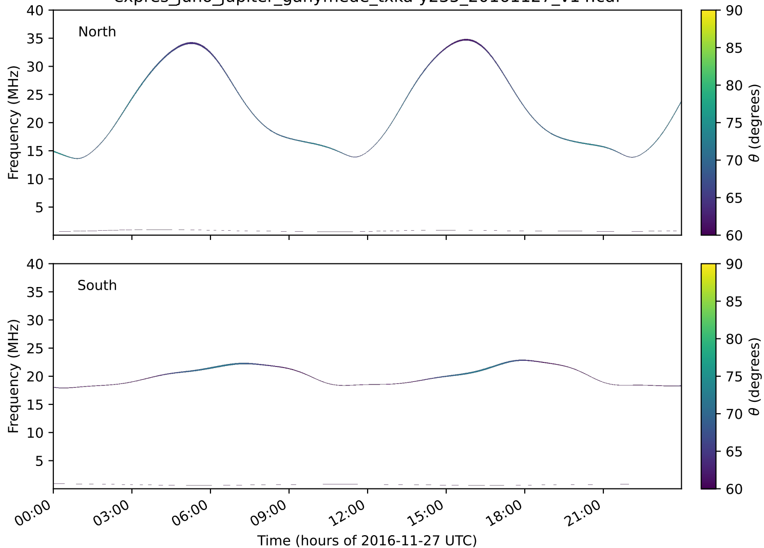
expres_juno_jupiter_ganymede_txka-y235_20161127_v14.cdf
