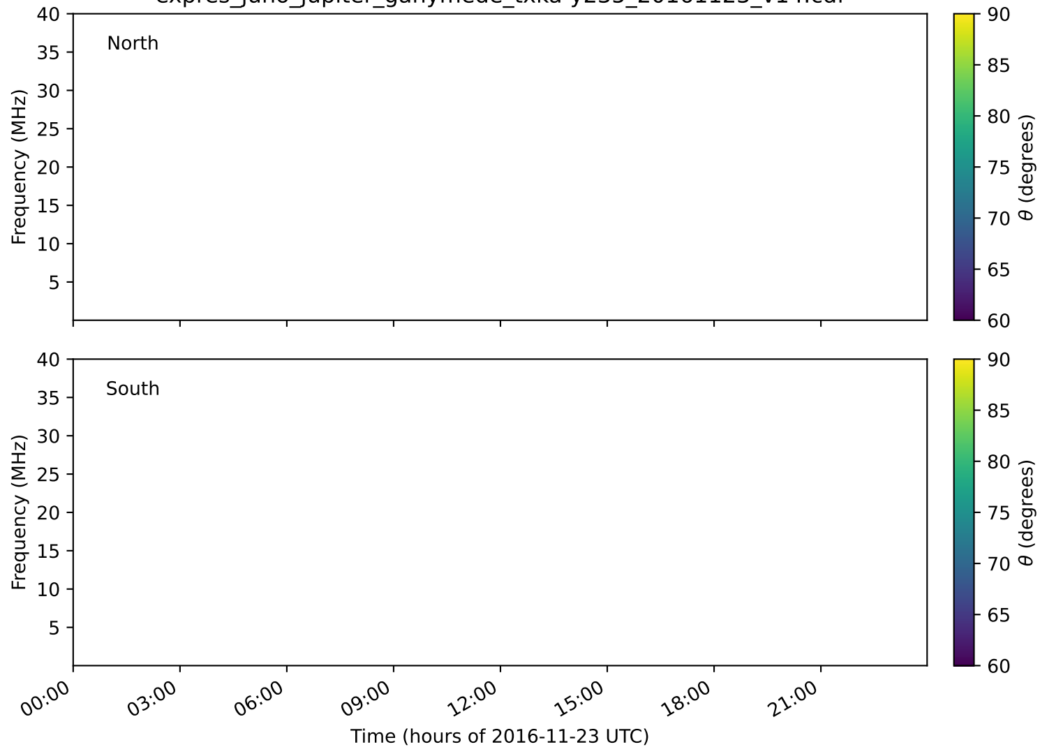
expres_juno_jupiter_ganymede_txka-y235_20161123_v14.cdf
