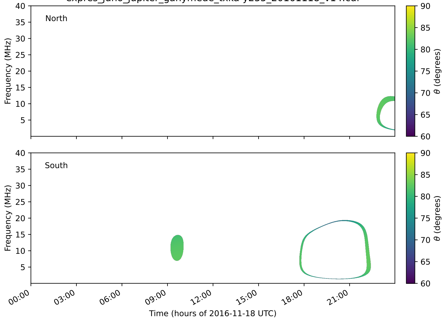
expres_juno_jupiter_ganymede_txka-y235_20161118_v14.cdf
