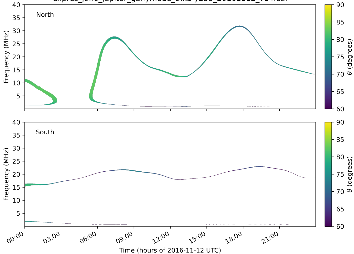
expres_juno_jupiter_ganymede_txka-y235_20161112_v14.cdf
