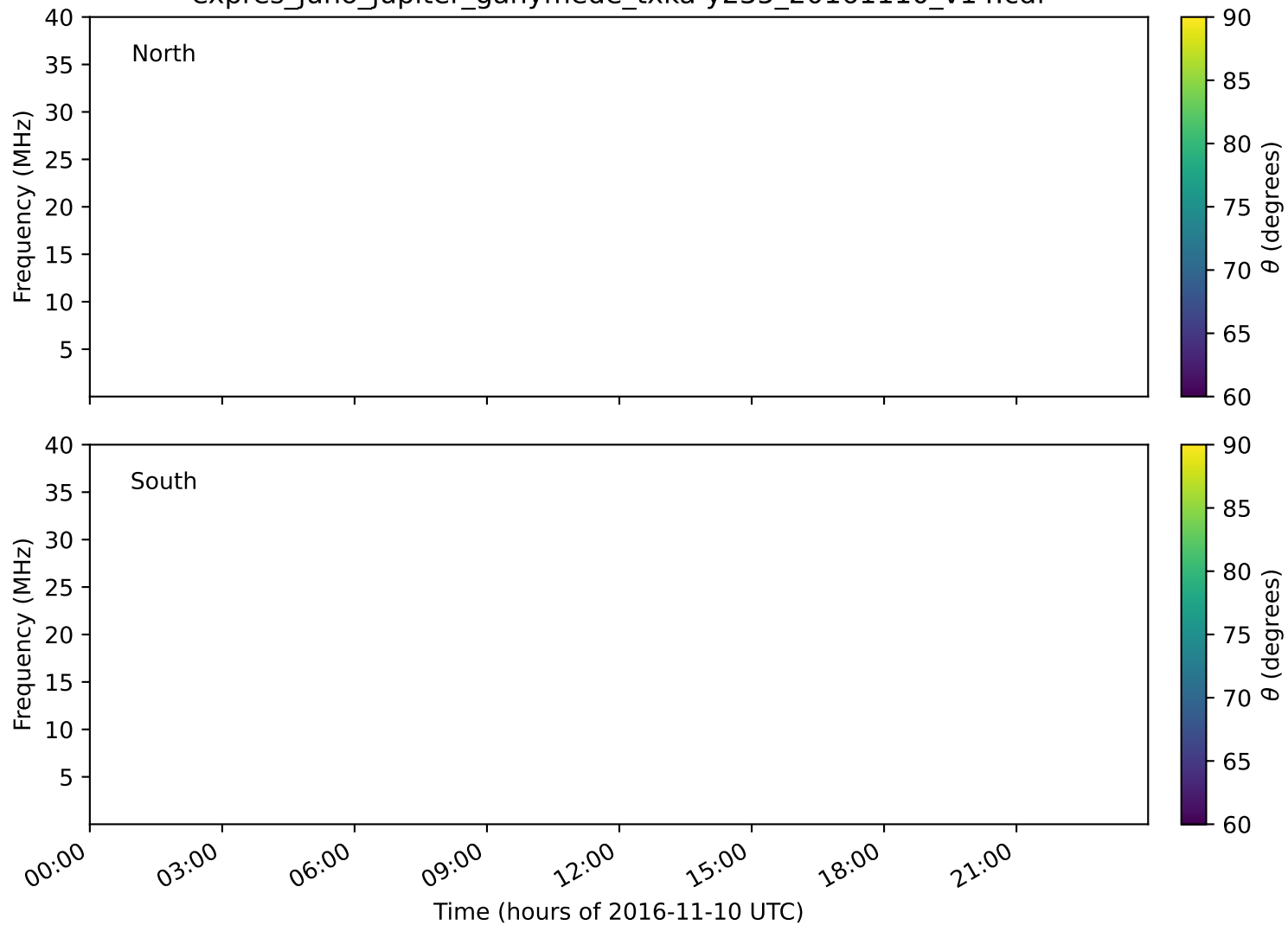
expres_juno_jupiter_ganymede_txka-y235_20161110_v14.cdf
