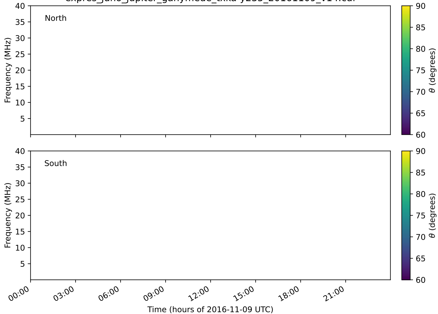
expres_juno_jupiter_ganymede_txka-y235_20161109_v14.cdf
