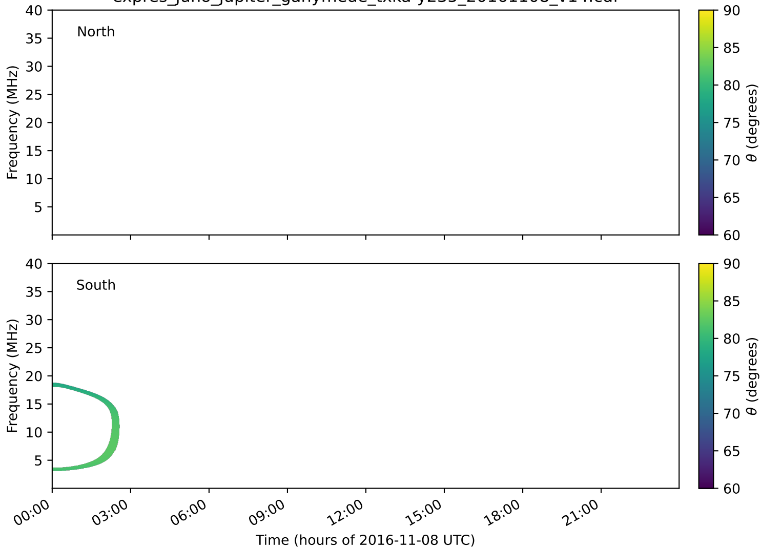
expres_juno_jupiter_ganymede_txka-y235_20161108_v14.cdf
