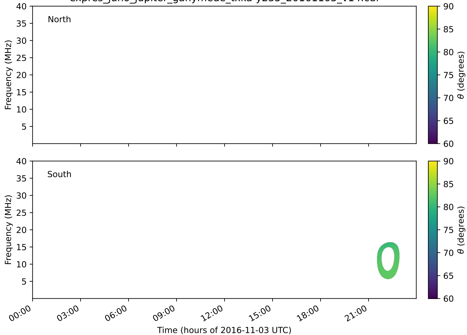
expres_juno_jupiter_ganymede_txka-y235_20161103_v14.cdf
