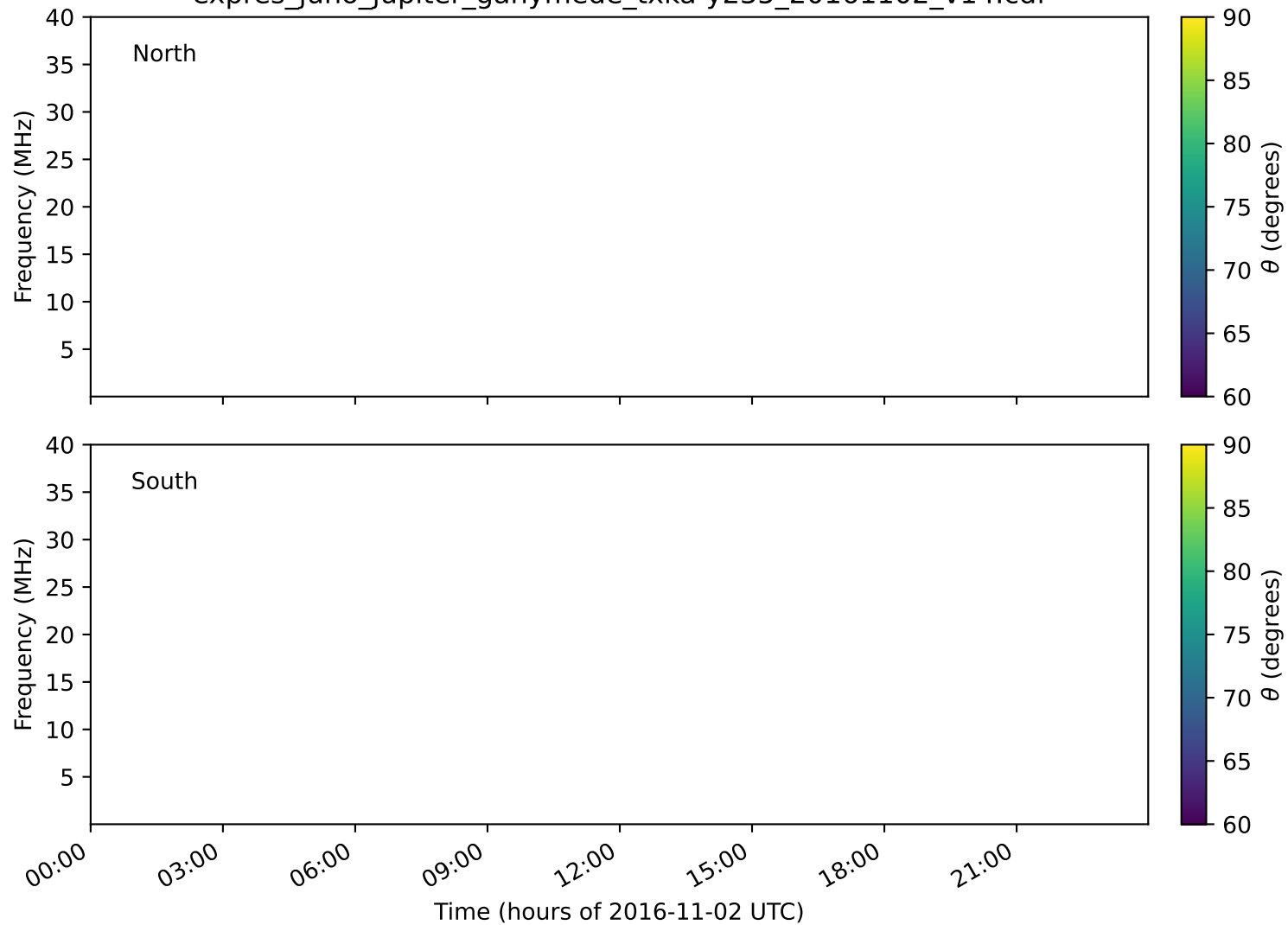
expres_juno_jupiter_ganymede_txka-y235_20161102_v14.cdf
