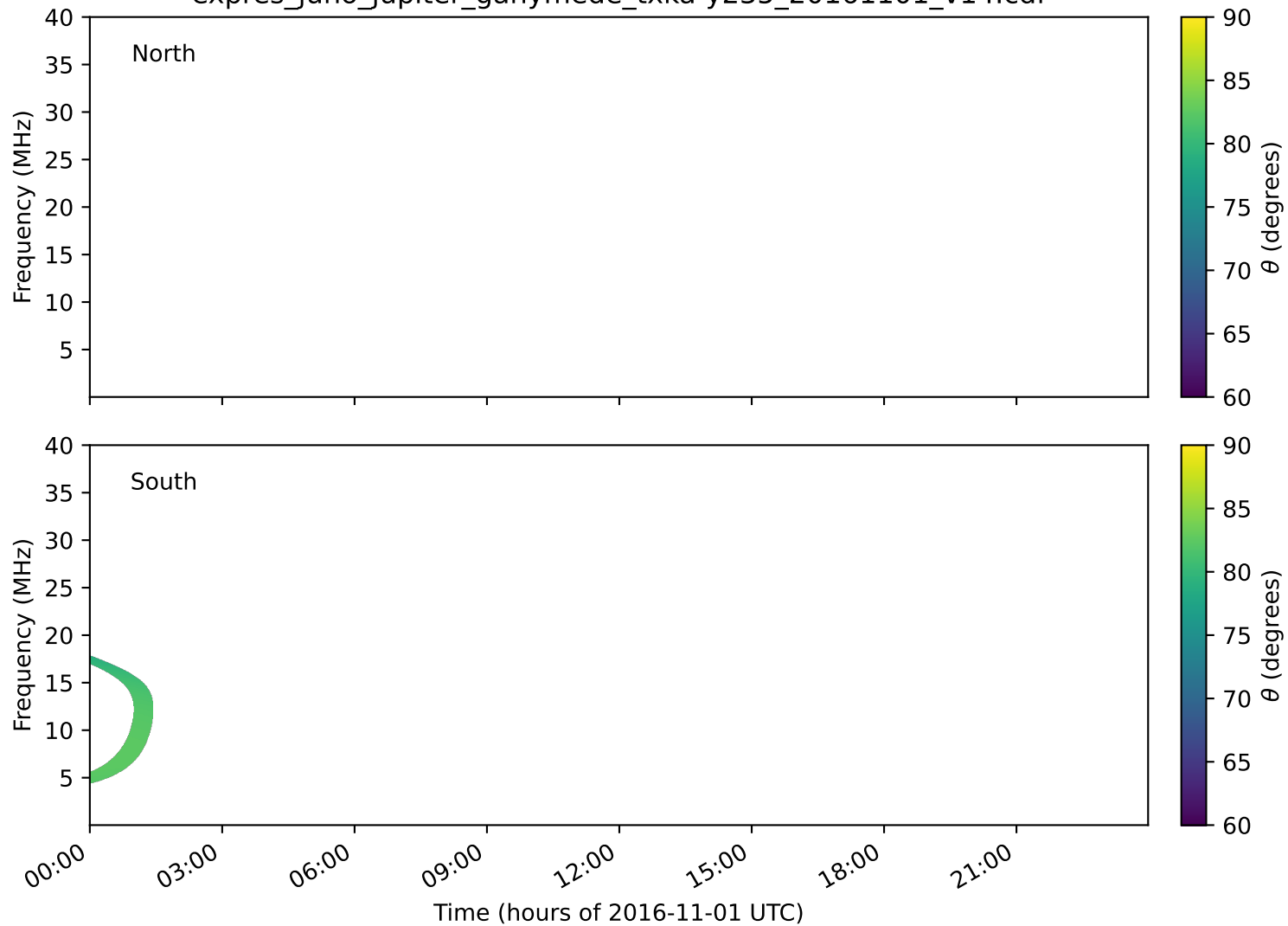
expres_juno_jupiter_ganymede_txka-y235_20161101_v14.cdf
