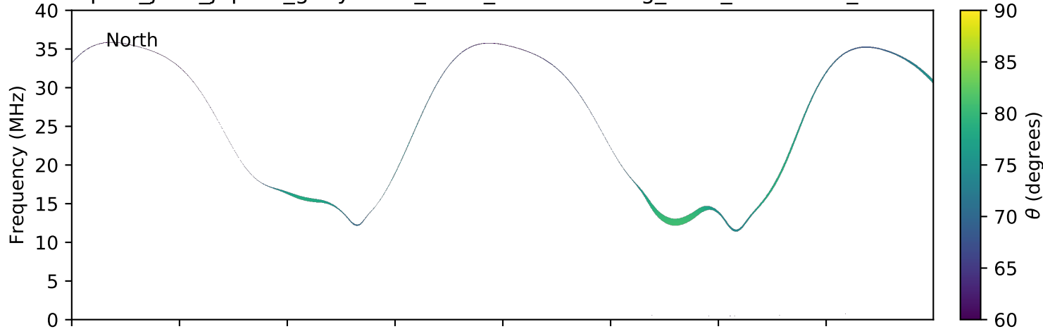
expres_juno_jupiter_ganymede_isaac_lossc-wid1deg_3kev_20161128_v01.cdf
