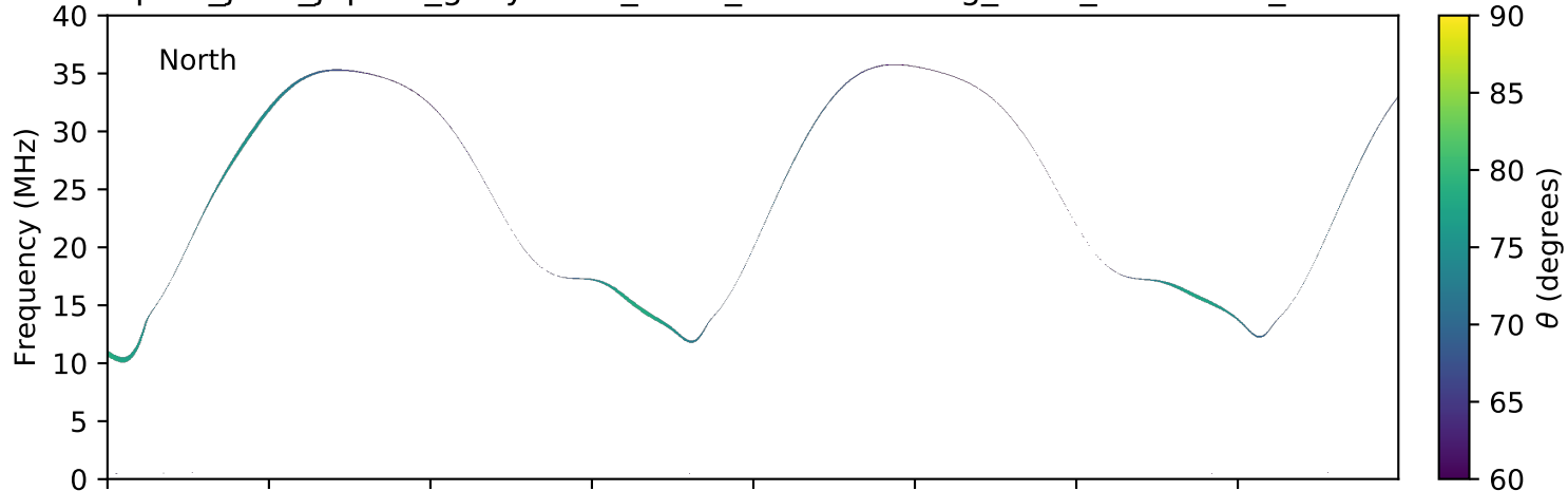
expres_juno_jupiter_ganymede_isaac_lossc-wid1deg_3kev_20161127_v01.cdf
