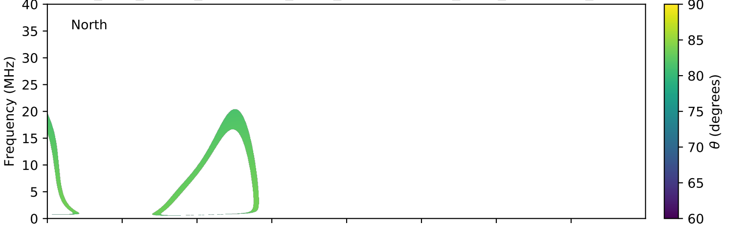
expres_juno_jupiter_ganymede_isaac_lossc-wid1deg_3kev_20161122_v01.cdf
