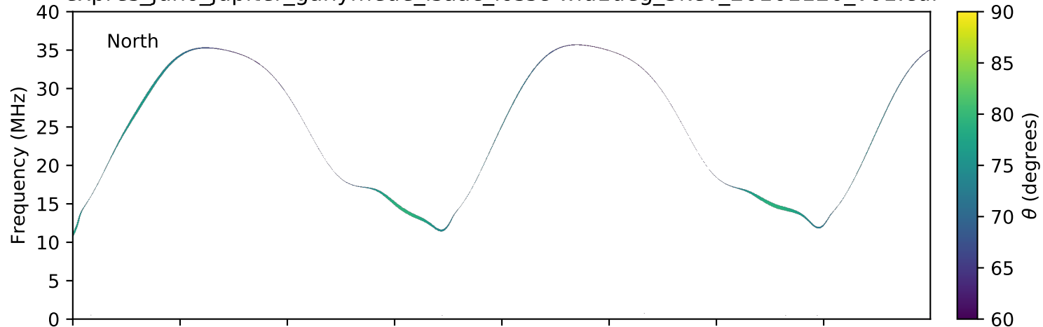
expres_juno_jupiter_ganymede_isaac_lossc-wid1deg_3kev_20161120_v01.cdf
