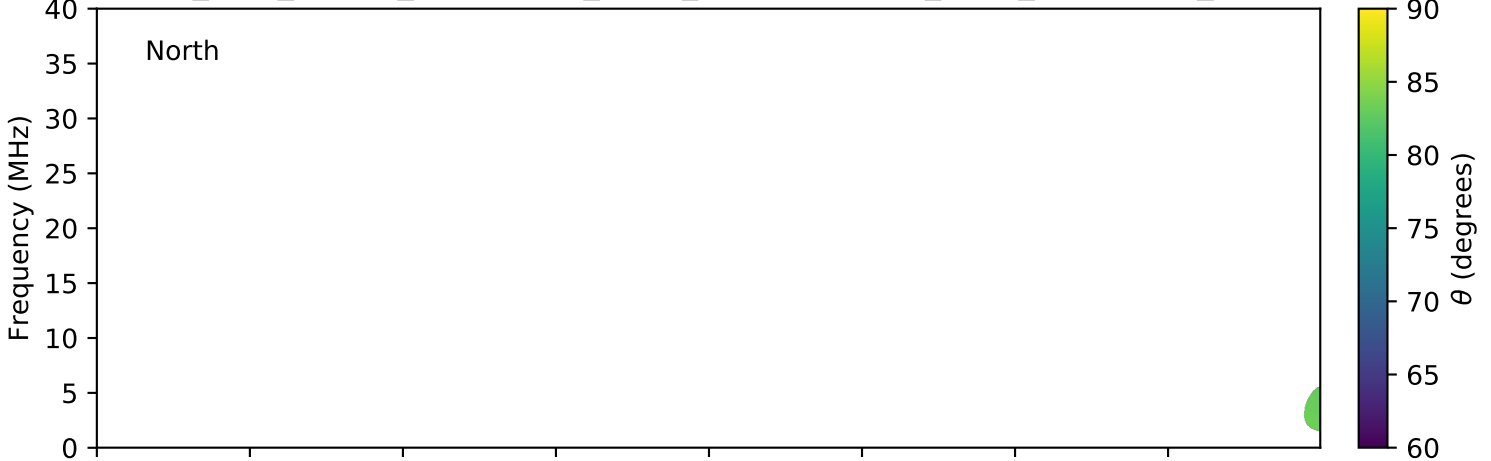
expres_juno_jupiter_ganymede_isaac_lossc-wid1deg_3kev_20161118_v01.cdf
