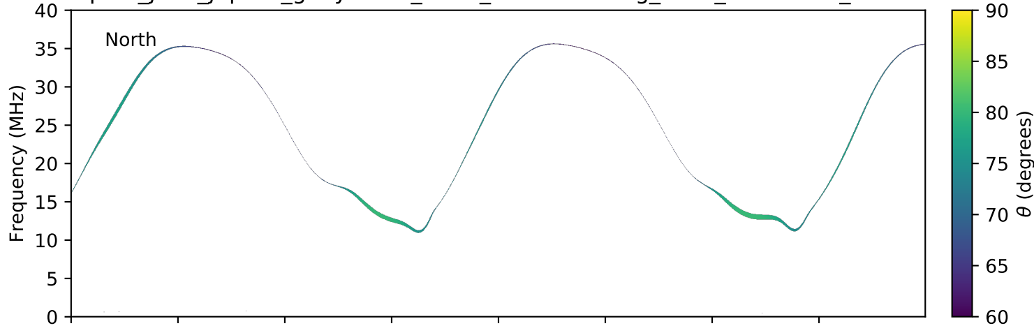
expres_juno_jupiter_ganymede_isaac_lossc-wid1deg_3kev_20161113_v01.cdf
