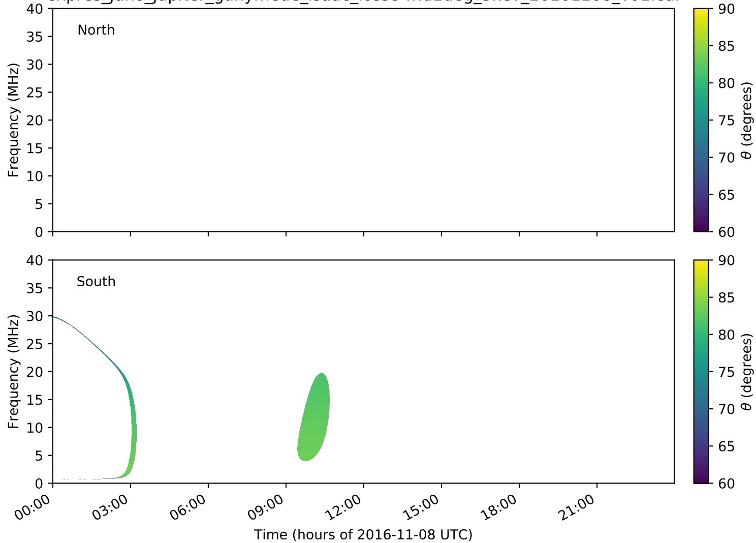
expres_juno_jupiter_ganymede_isaac_lossc-wid1deg_3kev_20161108_v01.cdf
