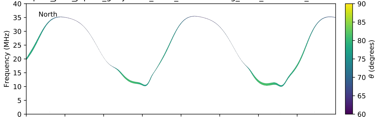
expres_juno_jupiter_ganymede_isaac_lossc-wid1deg_3kev_20161106_v01.cdf
