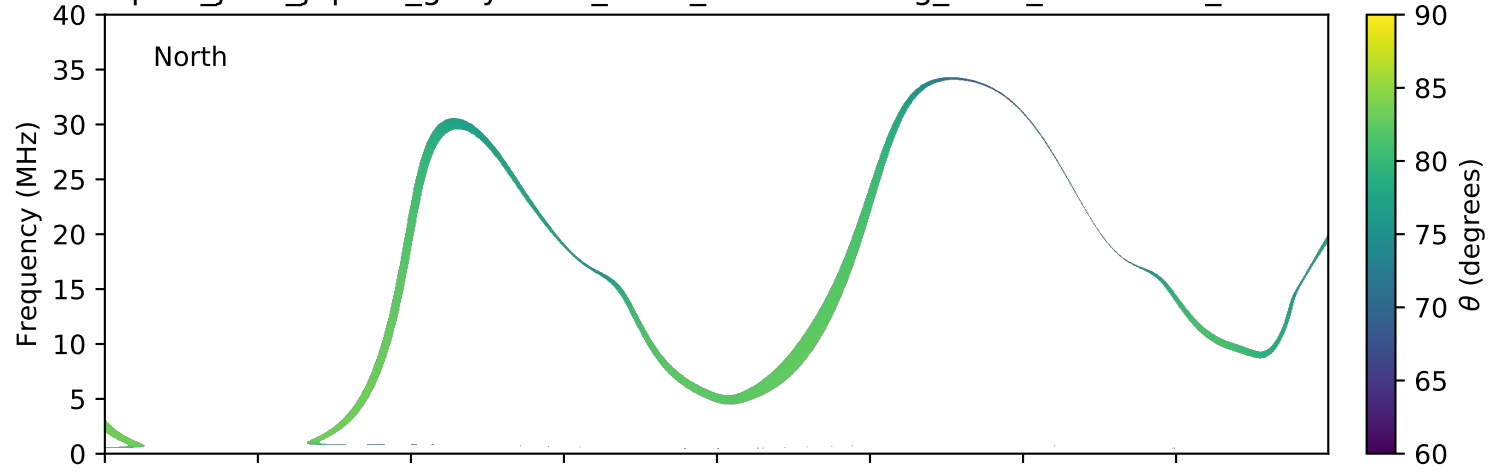
expres_juno_jupiter_ganymede_isaac_lossc-wid1deg_3kev_20161105_v01.cdf
