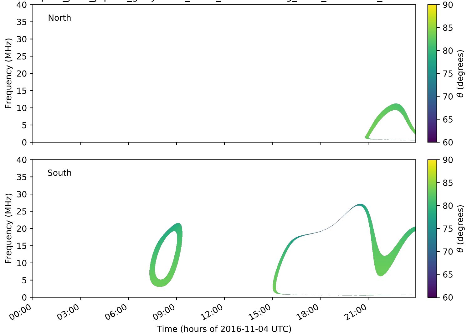
expres_juno_jupiter_ganymede_isaac_lossc-wid1deg_3kev_20161104_v01.cdf
