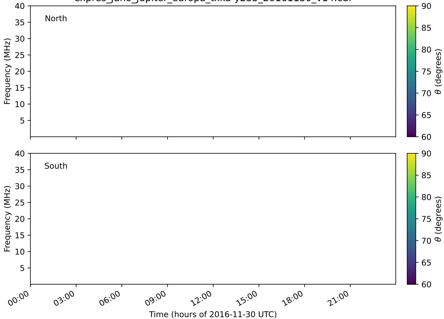
expres_juno_jupiter_europa_txka-y235_20161130_v14.cdf
