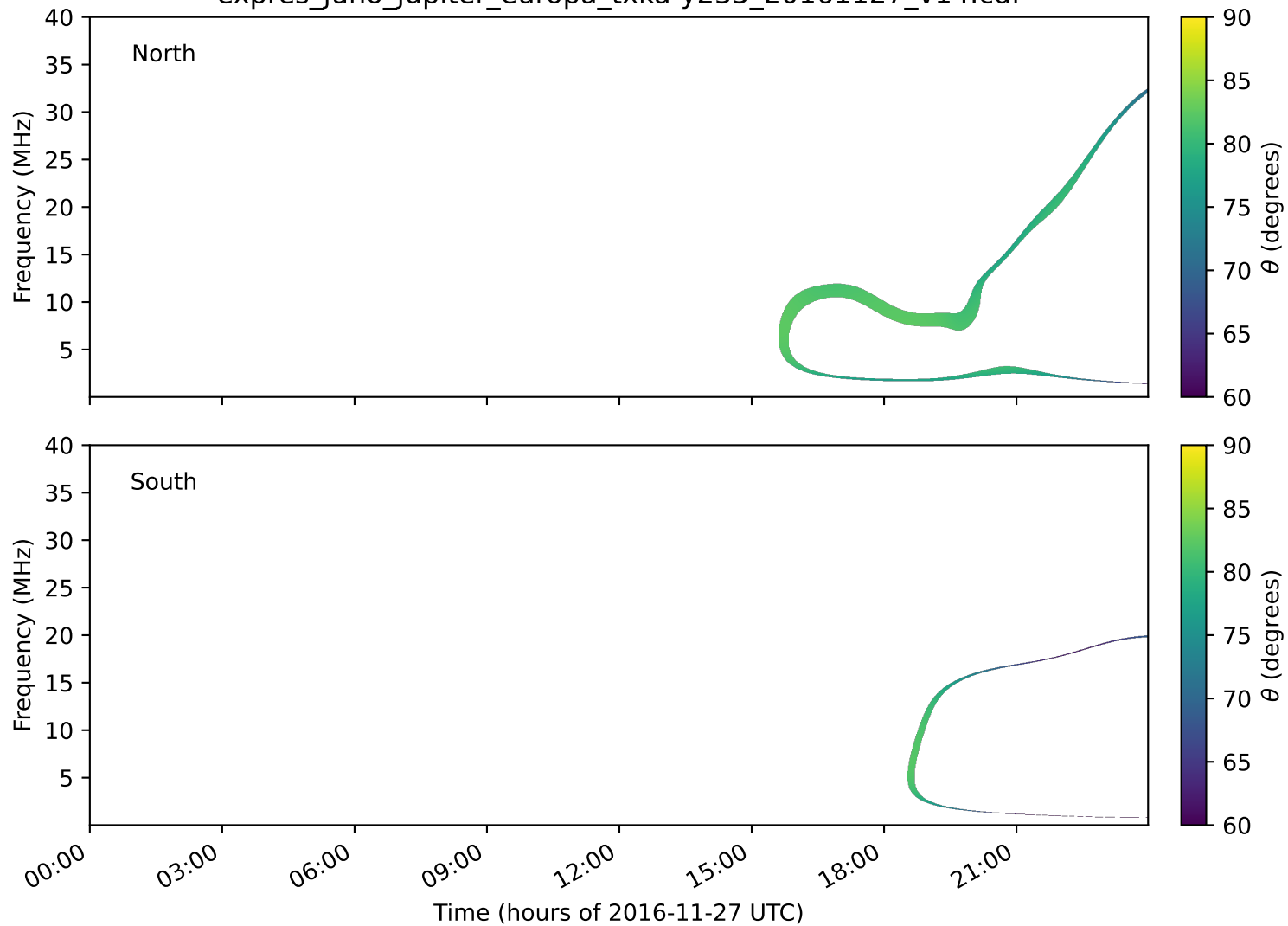
expres_juno_jupiter_europa_txka-y235_20161127_v14.cdf
