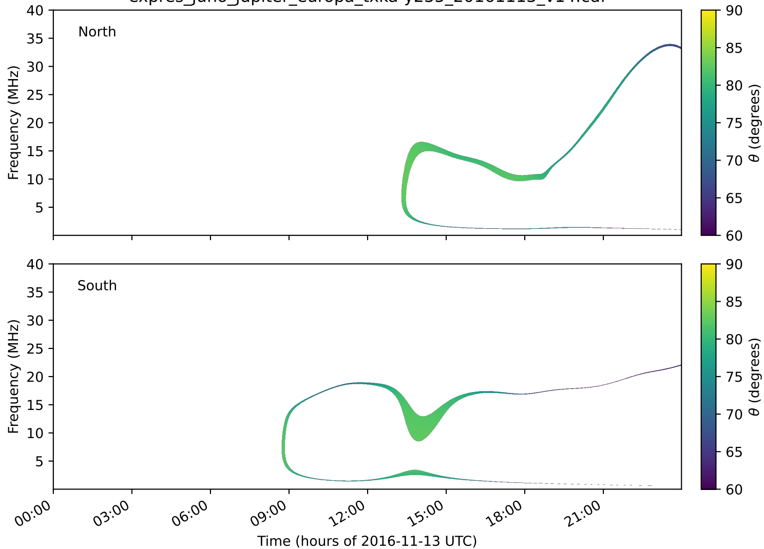
expres_juno_jupiter_europa_txka-y235_20161113_v14.cdf
