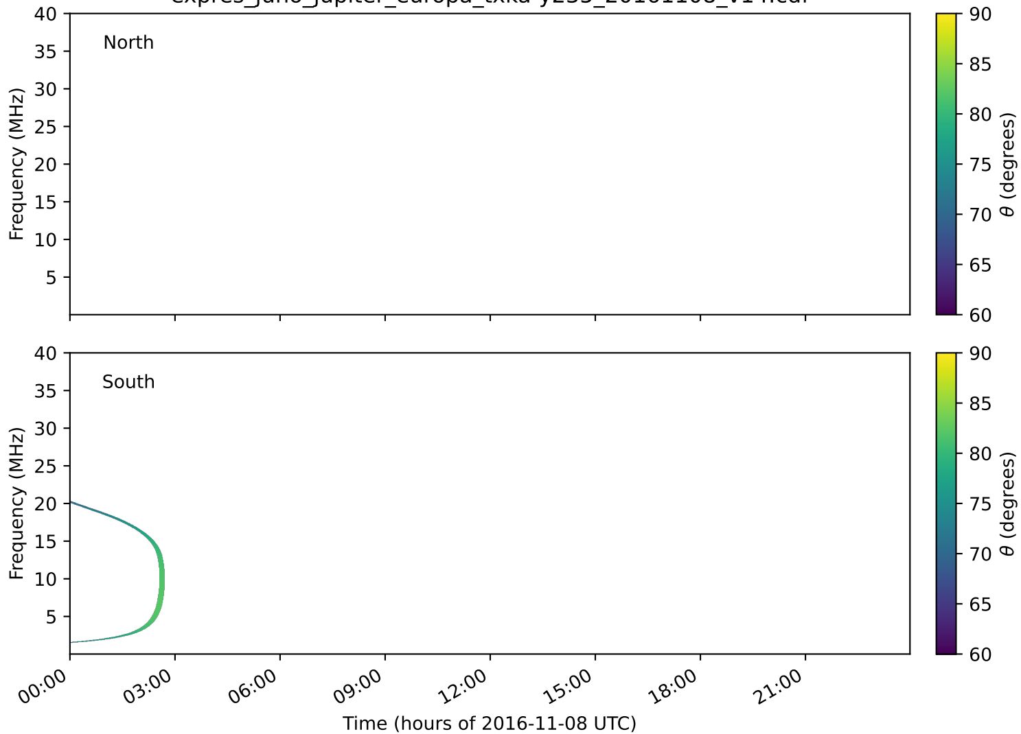
expres_juno_jupiter_europa_txka-y235_20161108_v14.cdf
