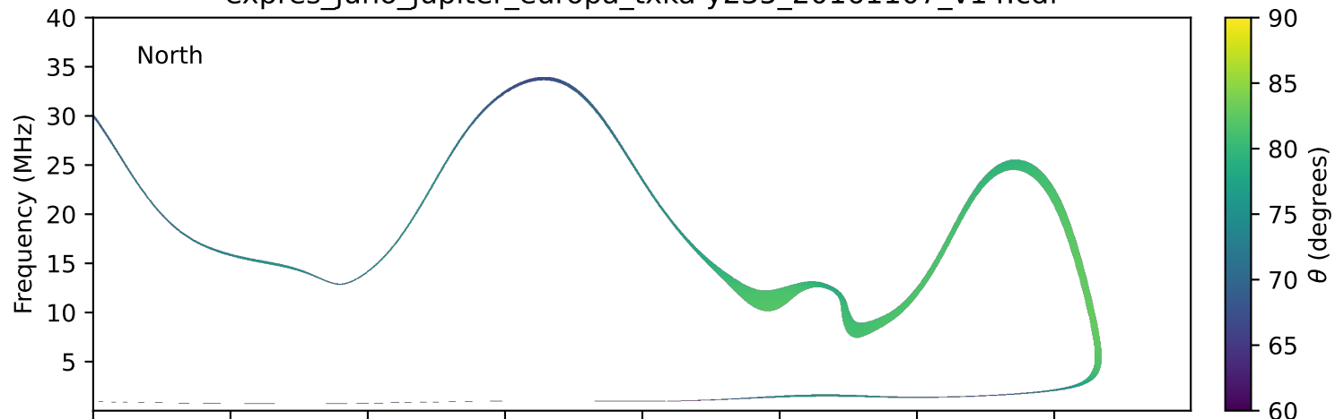
expres_juno_jupiter_europa_txka-y235_20161107_v14.cdf
