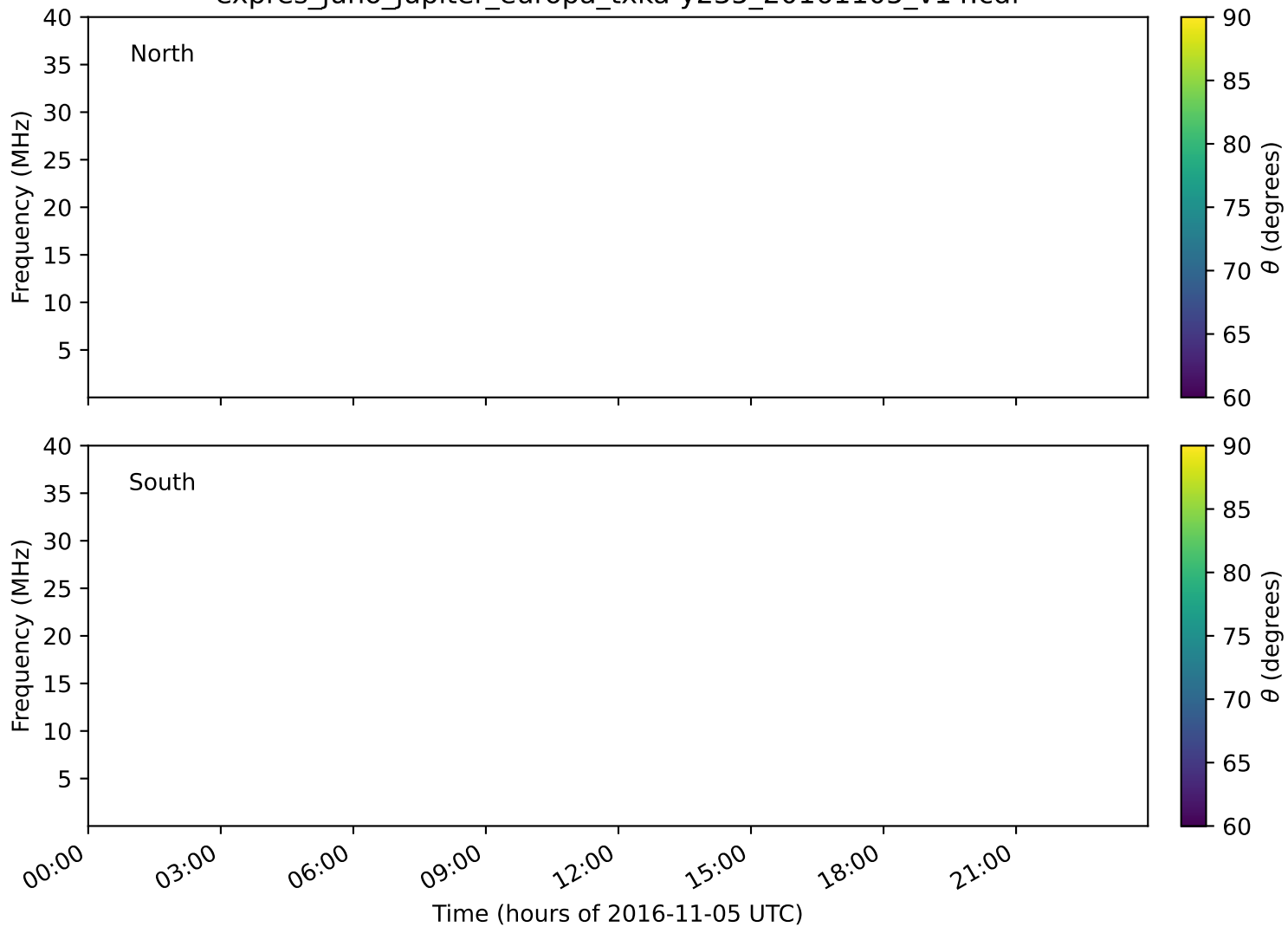
expres_juno_jupiter_europa_txka-y235_20161105_v14.cdf
