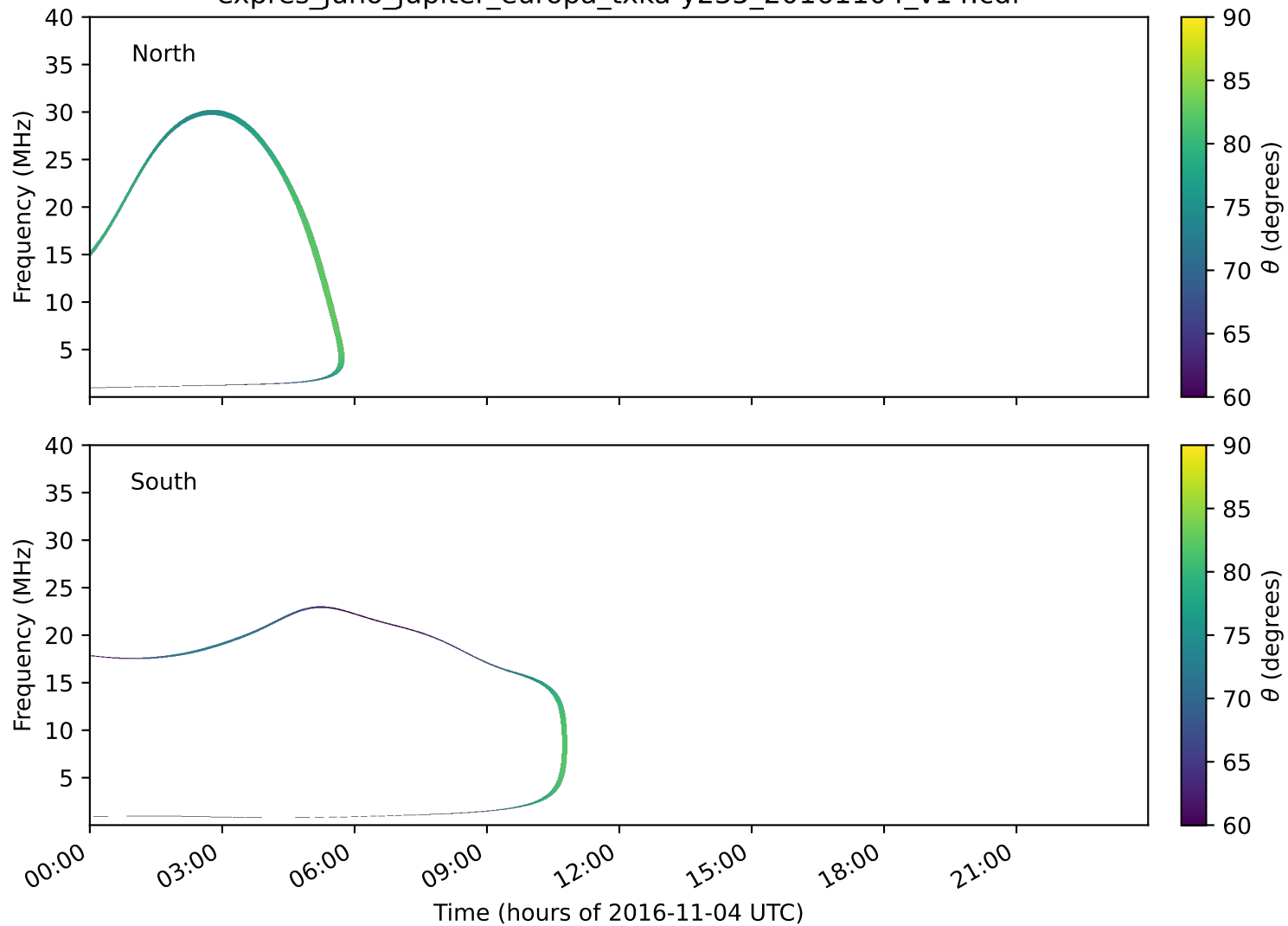
expres_juno_jupiter_europa_txka-y235_20161104_v14.cdf
