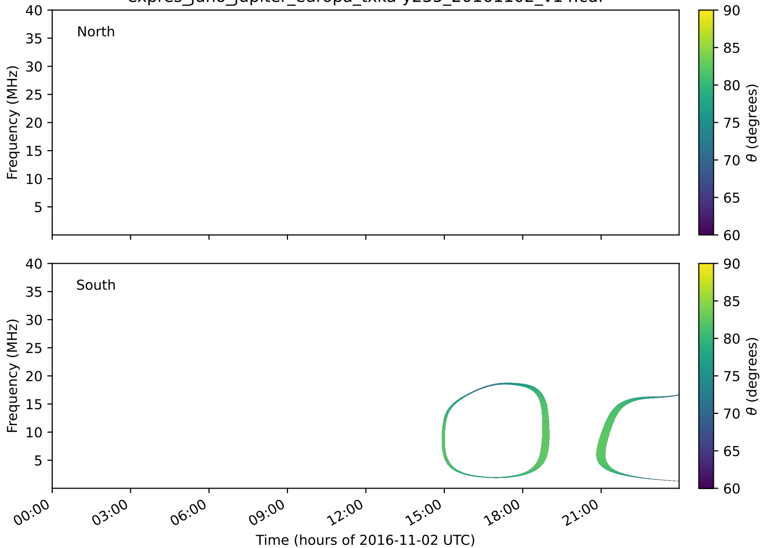
expres_juno_jupiter_europa_txka-y235_20161102_v14.cdf
