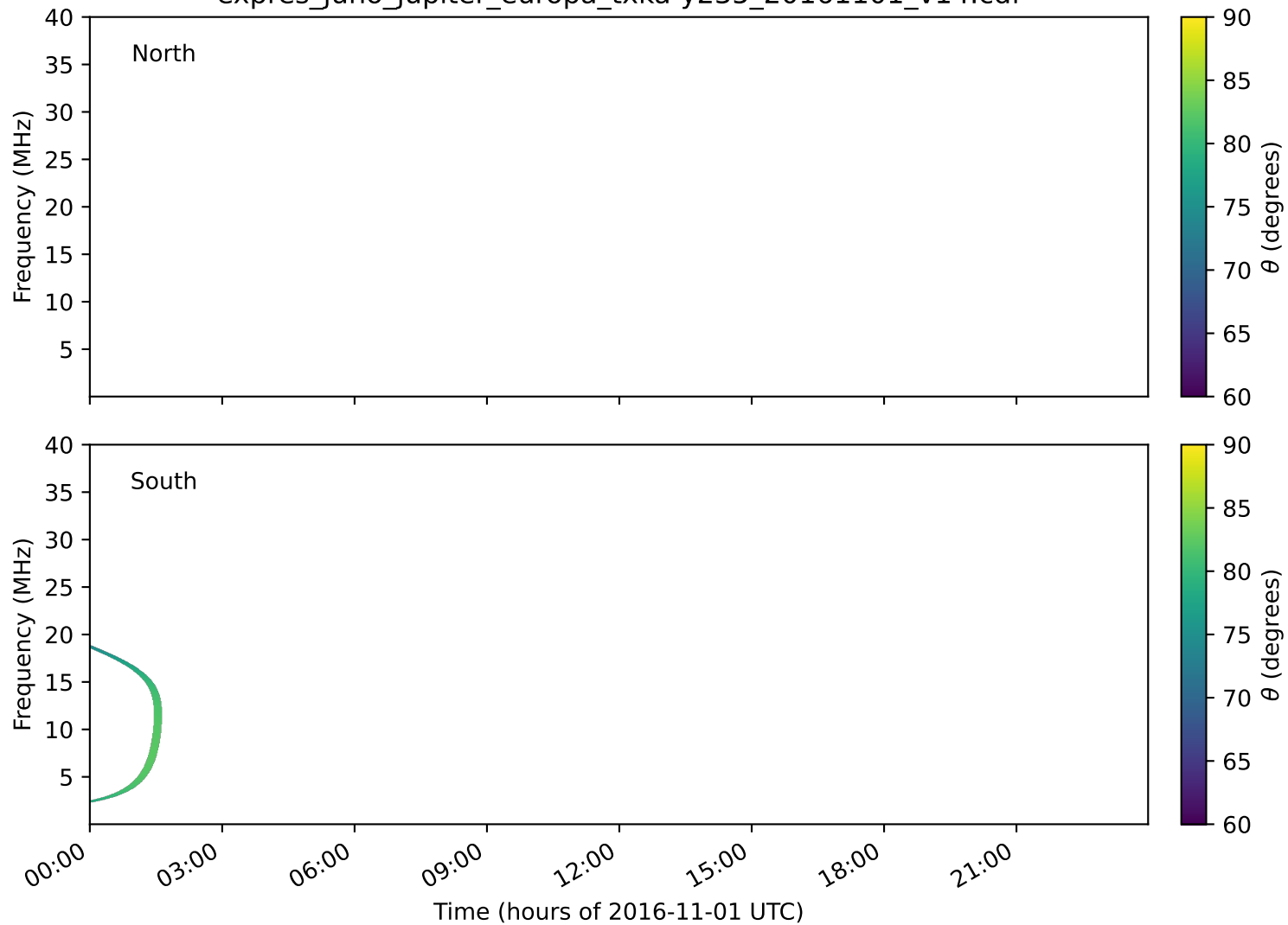
expres_juno_jupiter_europa_txka-y235_20161101_v14.cdf
