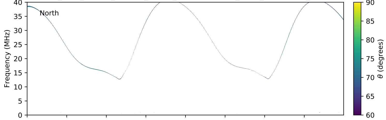
expres_juno_jupiter_europa_jrm09_lossc-wid1deg_3kev_20161128_v01.cdf
