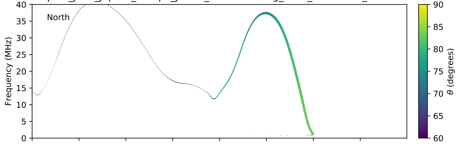
expres_juno_jupiter_europa_jrm09_lossc-wid1deg_3kev_20161125_v01.cdf
