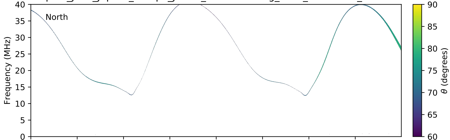
expres_juno_jupiter_europa_jrm09_lossc-wid1deg_3kev_20161121_v01.cdf
