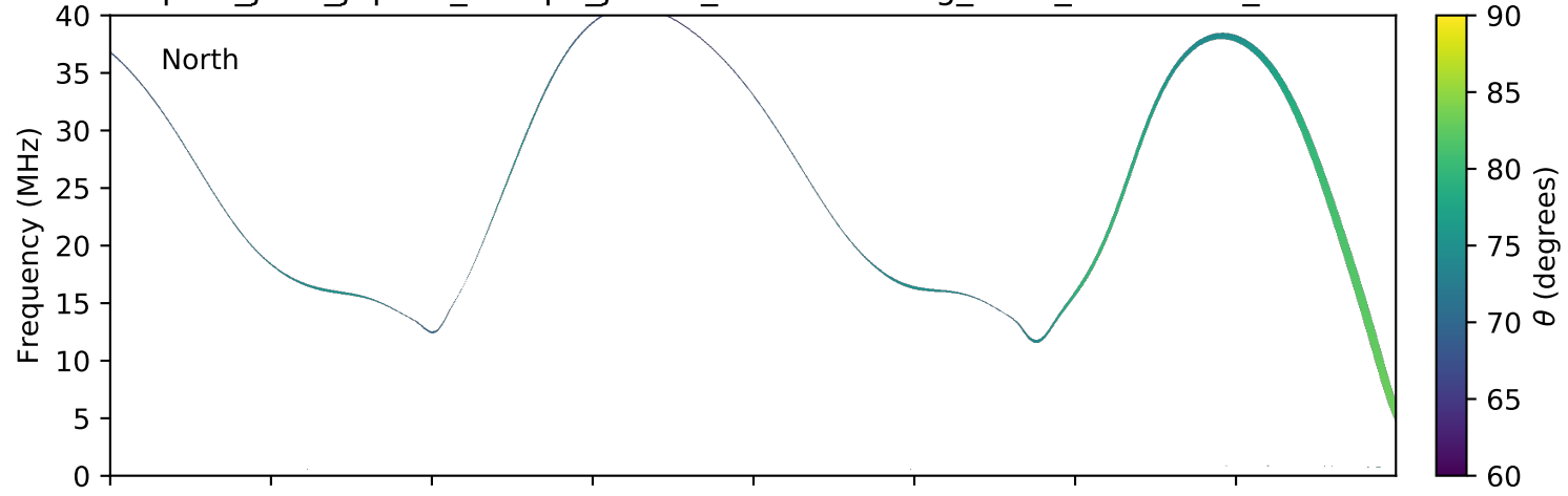
expres_juno_jupiter_europa_jrm09_lossc-wid1deg_3kev_20161114_v01.cdf
