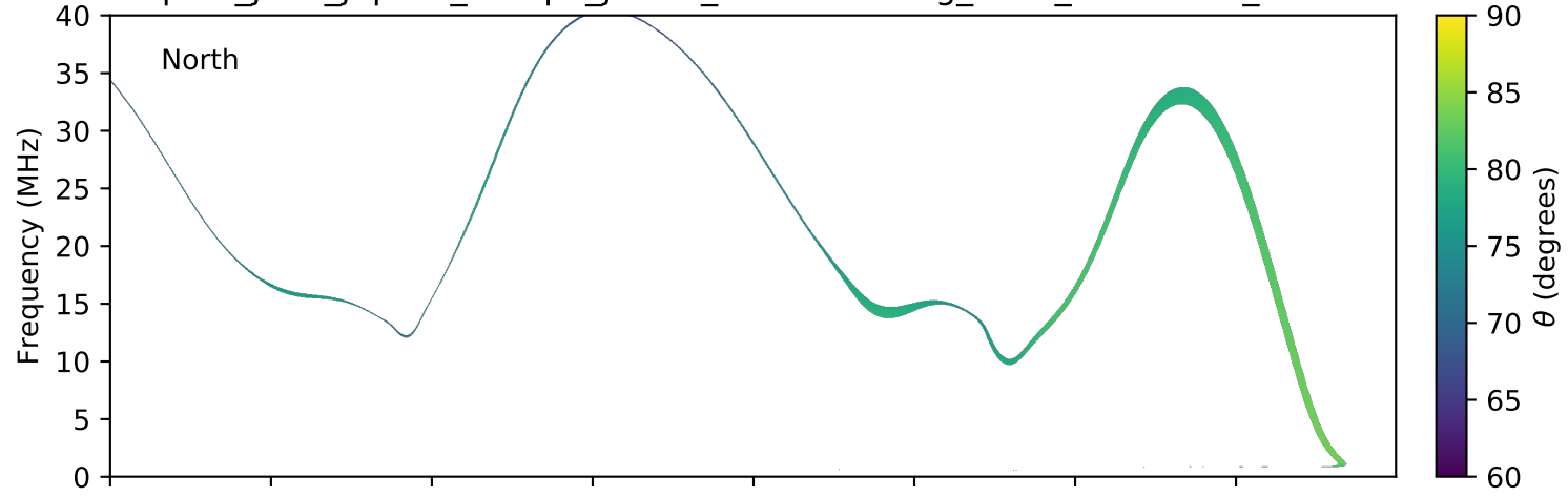
expres_juno_jupiter_europa_jrm09_lossc-wid1deg_3kev_20161107_v01.cdf
