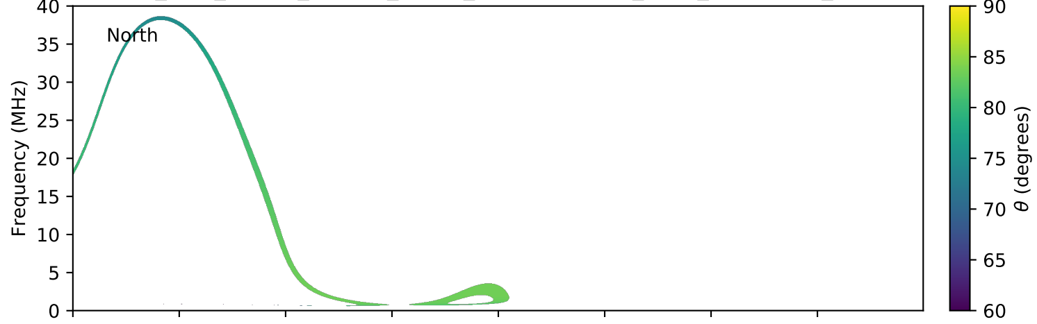
expres_juno_jupiter_europa_jrm09_lossc-wid1deg_3kev_20161104_v01.cdf
