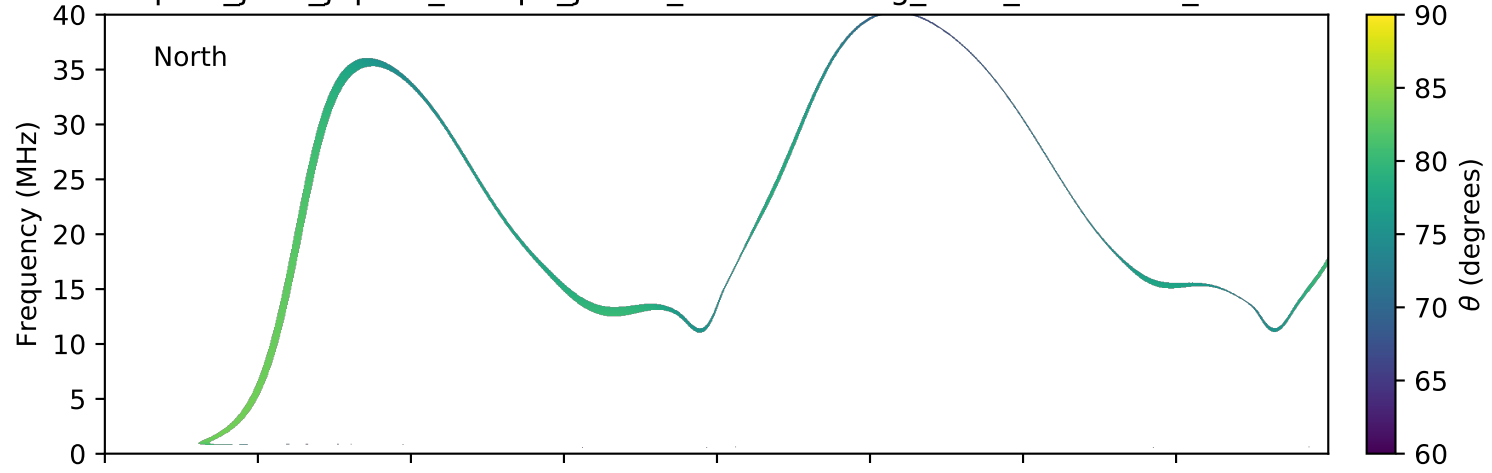
expres_juno_jupiter_europa_jrm09_lossc-wid1deg_3kev_20161103_v01.cdf
