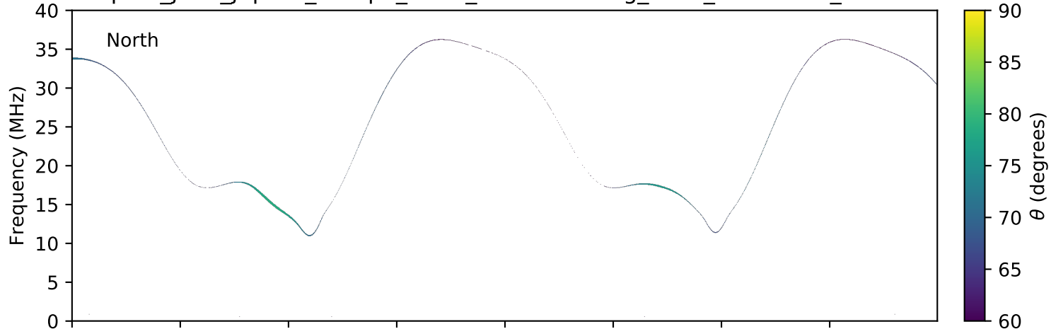
expres_juno_jupiter_europa_isaac_lossc-wid1deg_3kev_20161128_v01.cdf
