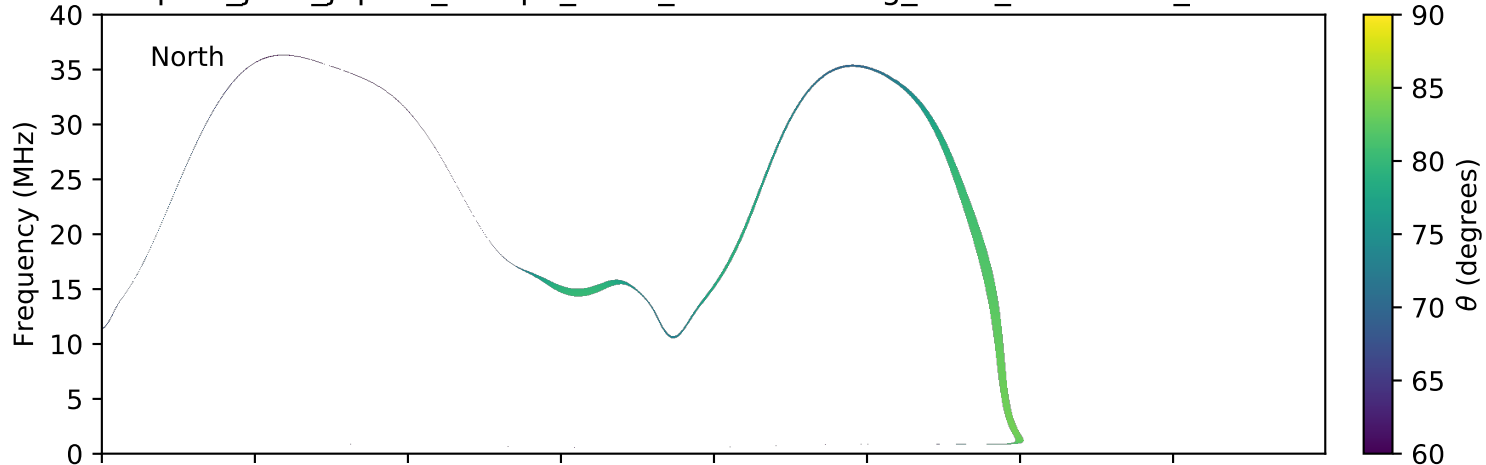
expres_juno_jupiter_europa_isaac_lossc-wid1deg_3kev_20161125_v01.cdf
